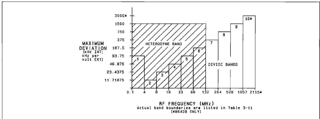
Figure 3-13. FM Deviation Limitations for each RF Frequency Band; Modulation Frequencies \geq 1389 Hz
