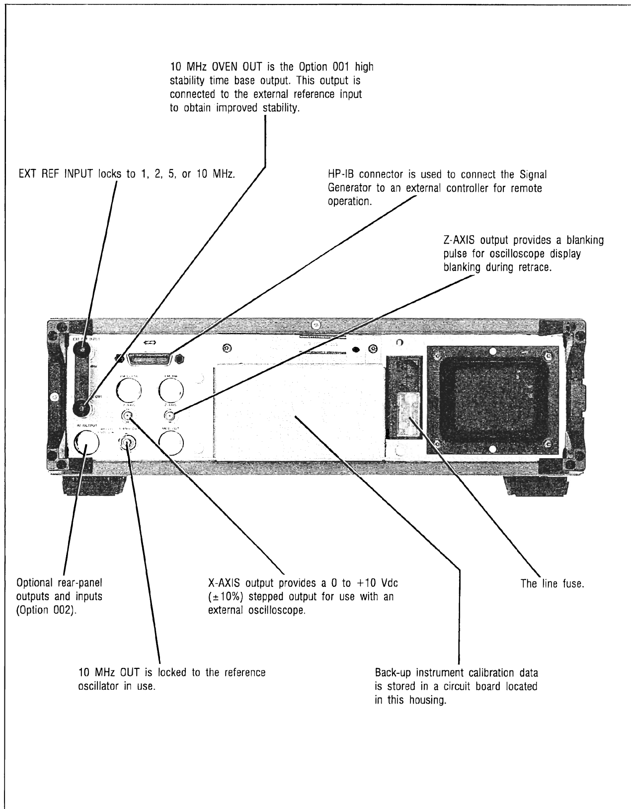
Figure 3-2. Rear-Panel Features
