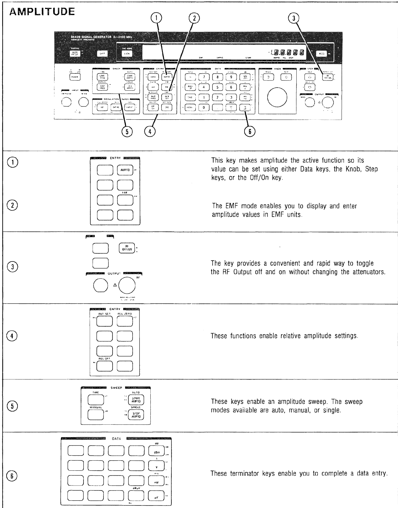
Figure 3-8. Amplitude-Related Functions
