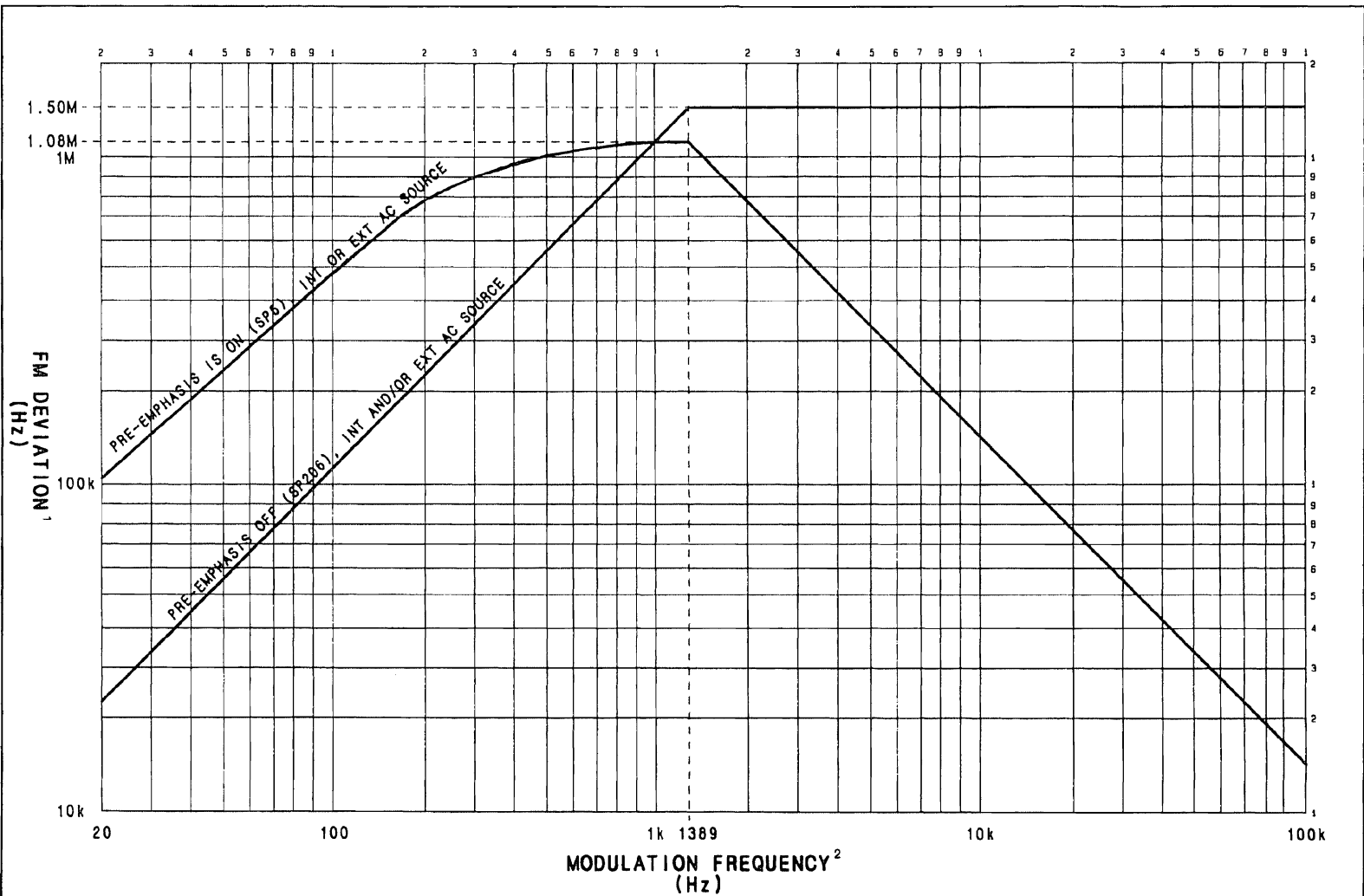
Figure 3-14. FM Deviation Limits with/without FM Pre-emphasis
